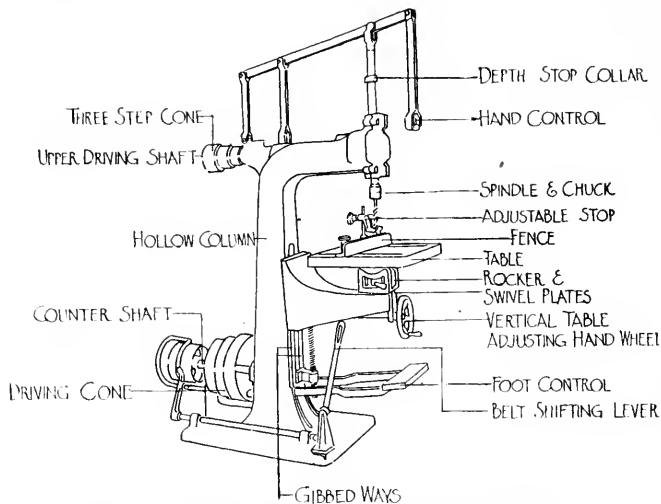
FIG. 191. VERTICAL SPINDLE BORING MACHINE.
